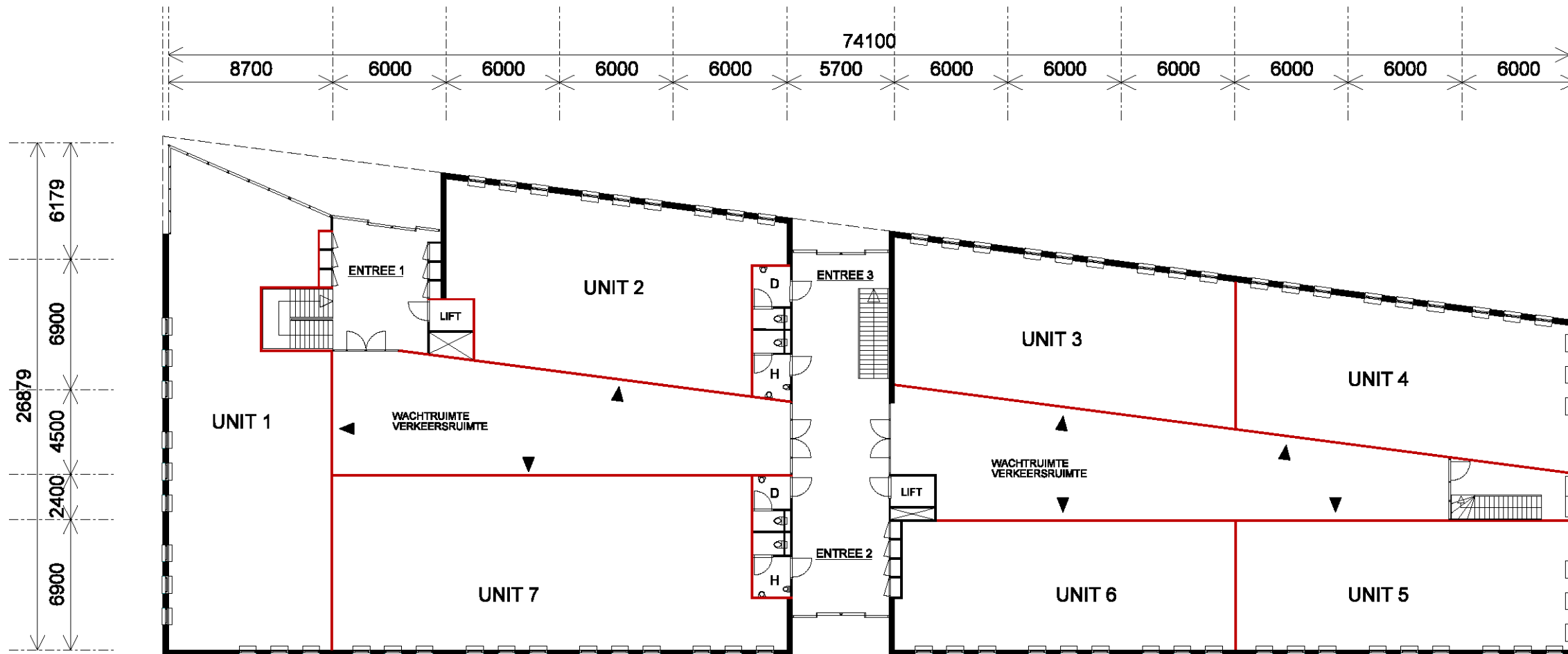
principe plattegrond begane grond
